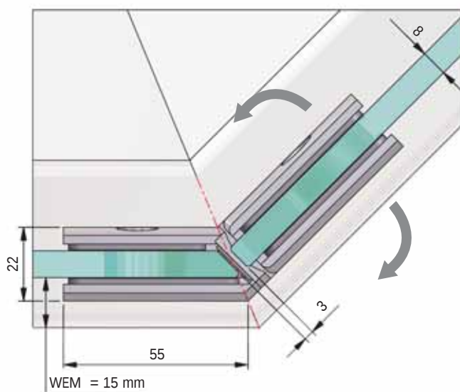
Türflügel beidseitig 90° öffnend/wing of the door opens in both directions 90°
