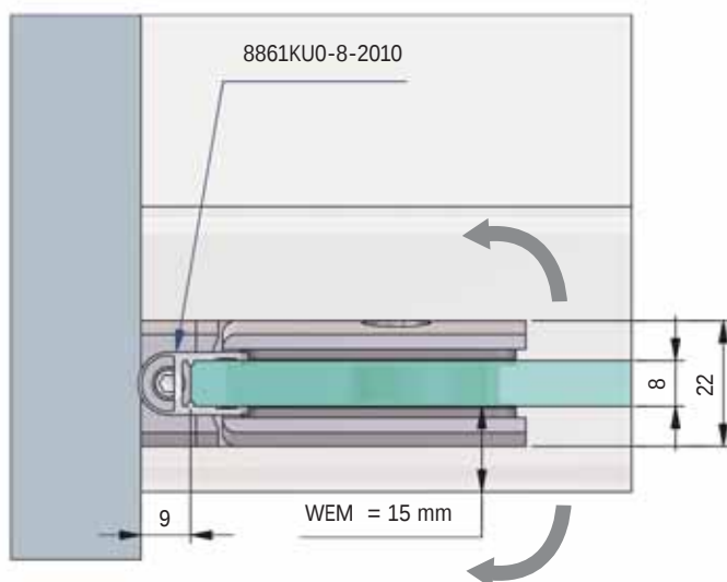
Türflügel beidseitig 90° öffnend/wing of the door opens in both directions 90°
