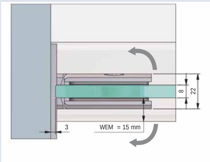
Türflügel beidseitig 90° öffnend/wing of the door opens in both directions 90°
