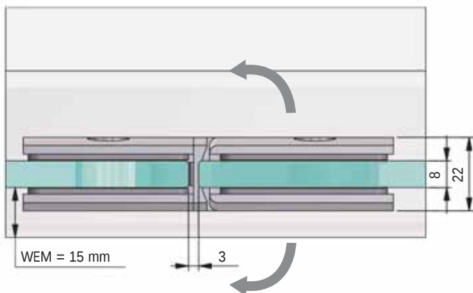
Türflügel beidseitig 90° öffnend/wing of the door opens in both directions 90°
