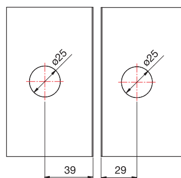
Scheibe A/panel A Scheibe B/panel B
