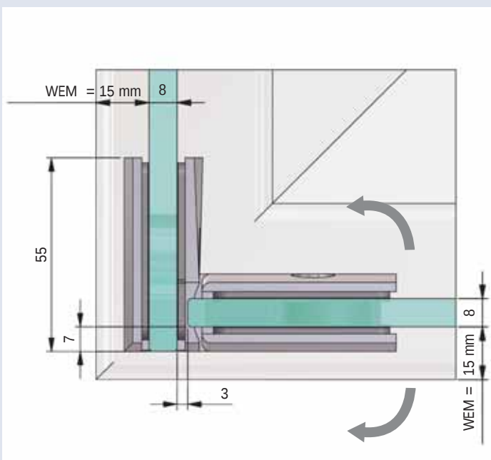
Türflügel beidseitig 90° öffnend/wing of the door opens in both directions 90°
