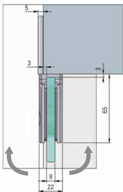
Türflügel beidseitig 90° öffnend/wing of the door opens in both directions 90°
